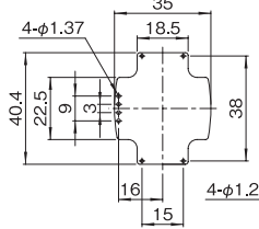
OAA/OAB-056□□-WT
