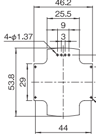
OAA/OAB-056□□-WT
