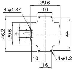
OAA/OAB-046□□-WT
