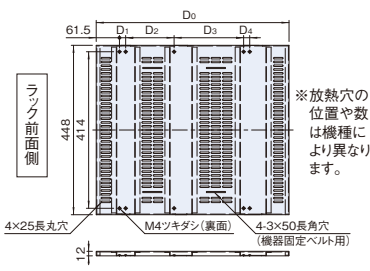
NPWS-44□□-H□
