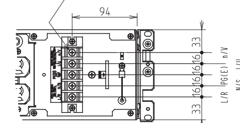
INSIDE VIEW OF TB COVER (REAR)
